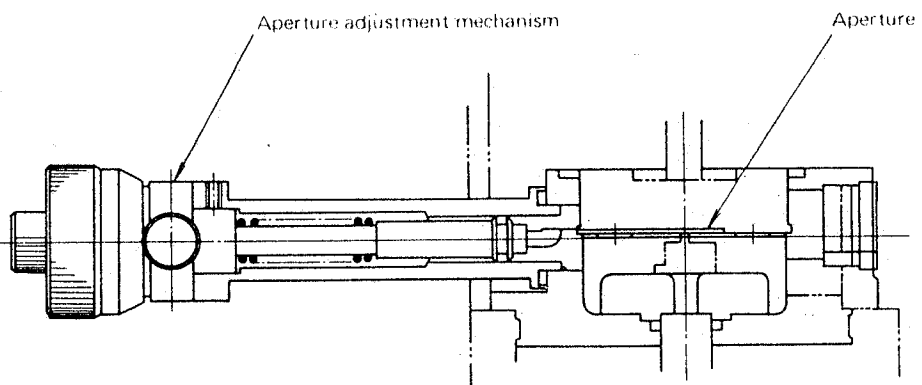
Fig. 3-7 Sectional View of Objective Lens Movable Aperture Assembly
